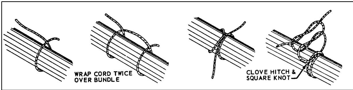
FIGURE 11-17. Making ties.
